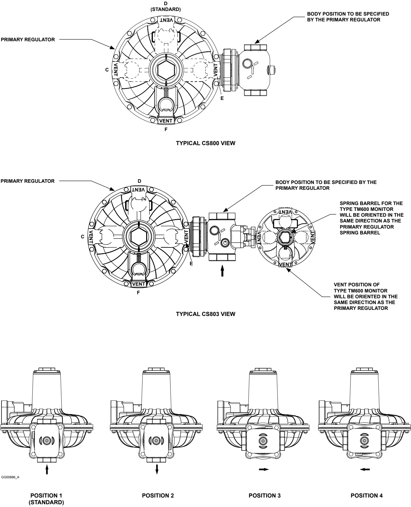
Figure 19. Spring Case Vent and Body Orientation
