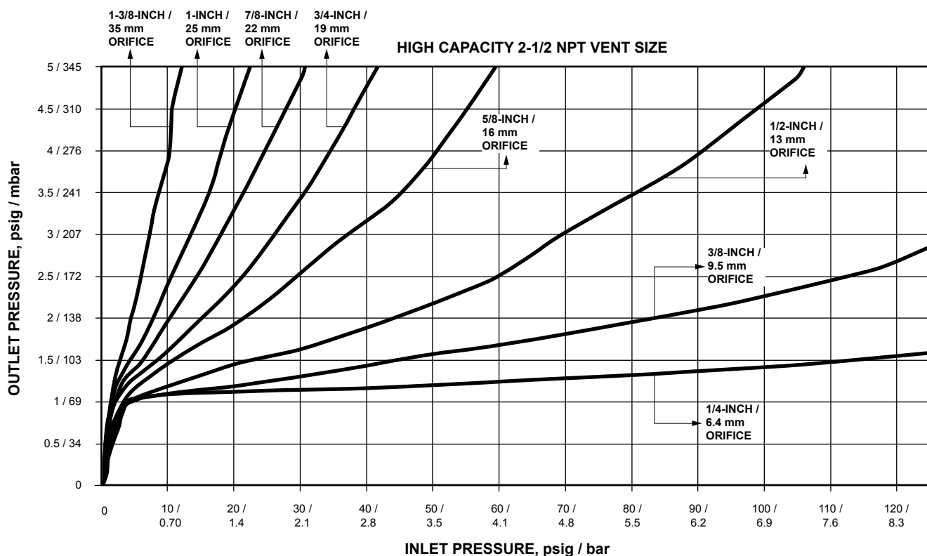
Figure 12. Type CS800IQ High Capacity Relief Curves (Blocked Open per Orifice Size) at 14 inches w.c. / 35 mbar Set Pressure
