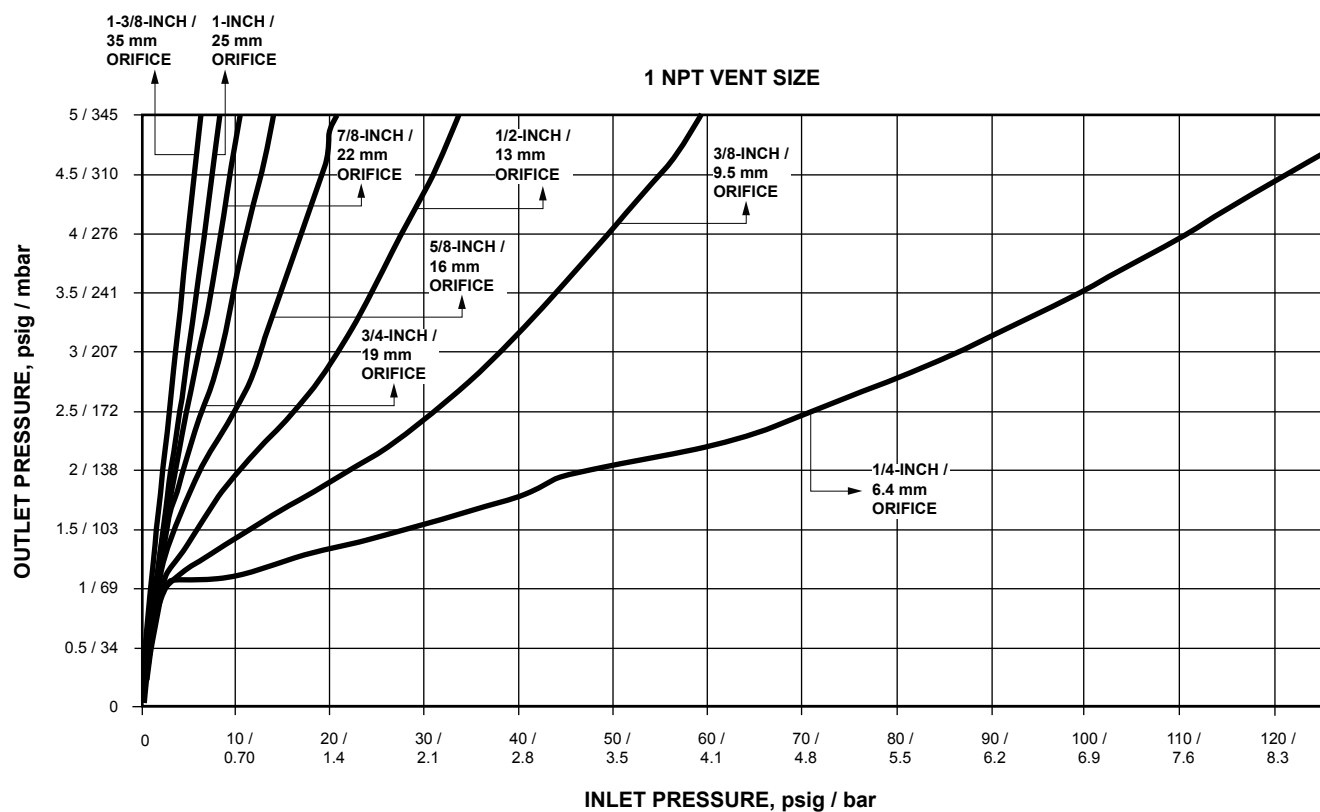
Figure 11. Type CS800IR Relief Curves (Blocked Open per Orifice Size) at 14 inches w.c. / 35 mbar Set Pressure
