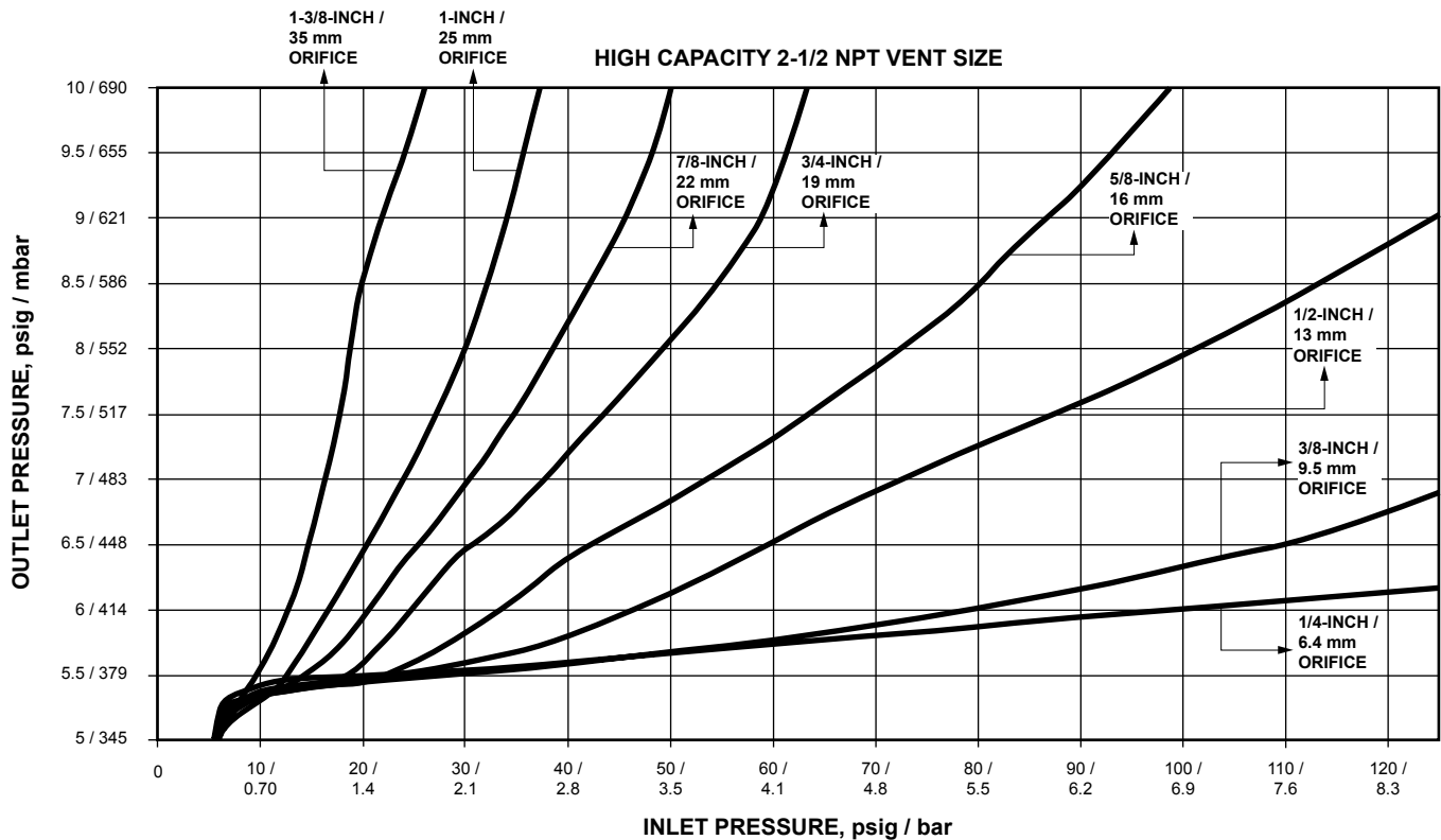
Figure 18. Type CS820IQ High Capacity Relief Curves (Blocked Open per Orifice Size) at 5 psig / 0.35 bar Set Pressure
