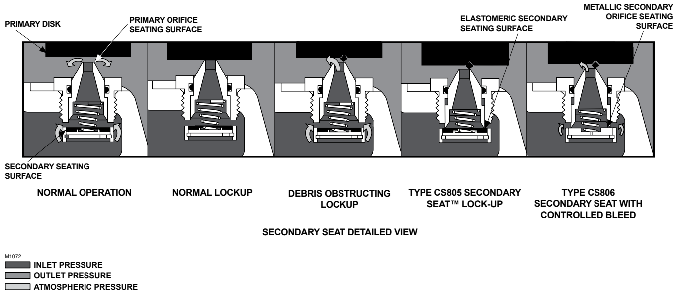
Figure 6. CS800 Series with Secondary Seat Protection (continued)
