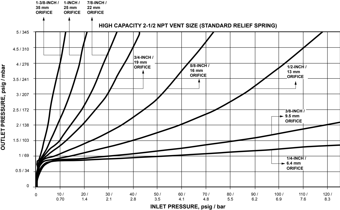
Figure 8. Type CS800IQ High Capacity Relief Curves (Blocked Open per Orifice Size) at 7 inches w.c. / 17 mbar Set Pressure
