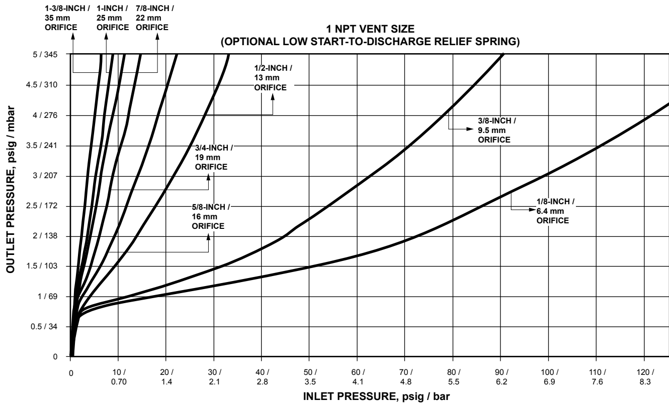
Figure 9. Type CS800IR Relief Curves (Blocked Open per Orifice Size) at 7 inches w.c. / 17 mbar Set Pressure
