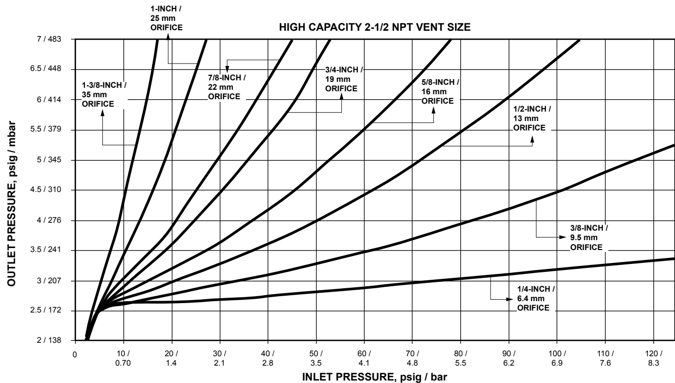
Figure 16. Type CS820IQ High Capacity Relief Curves (Blocked Open per Orifice Size) at 2 psig / 0.14 bar Set Pressure
