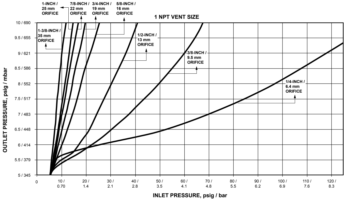
Figure 17. Type CS820IR Relief Curves (Blocked Open per Orifice Size) at 5 psig / 0.35 bar Set Pressure
