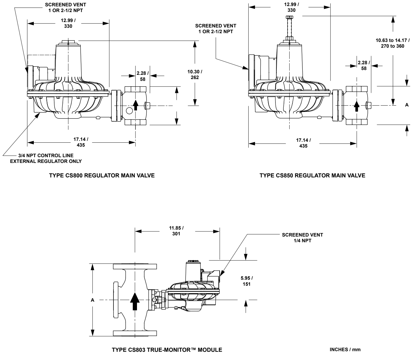
Figure 20. Dimensions
