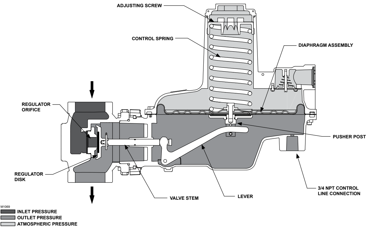
Figure 4. Type CS800EN Externally Registered Regulator Operational Schematic
