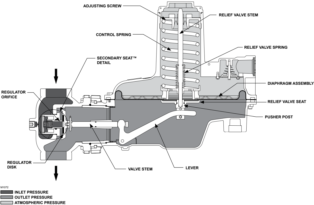
Figure 6. CS800 Series with Secondary Seat Protection
