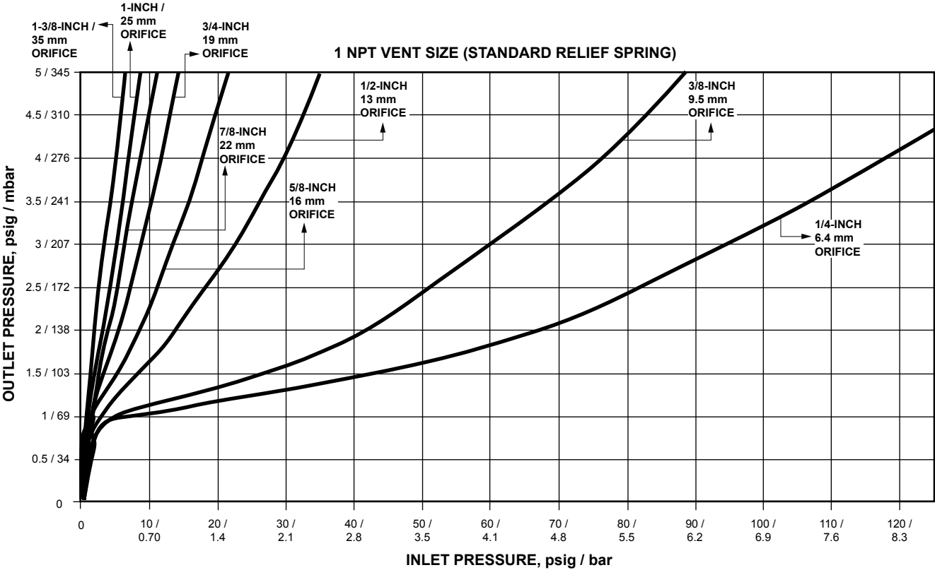
Figure 7. Type CS800IR Relief Curves (Blocked Open per Orifice Size) at 7 inches w.c. / 17 mbar Set Pressure
