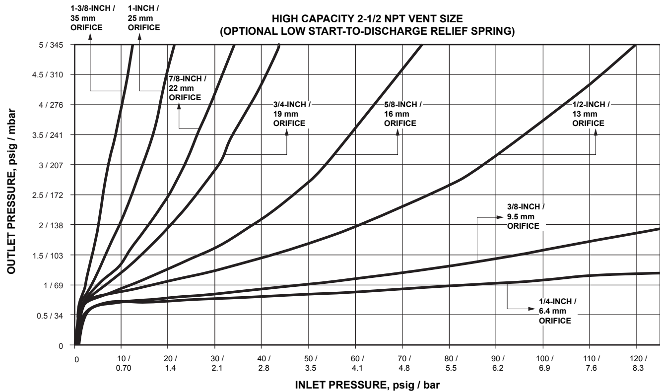
Figure 10. Type CS800IQ High Capacity Relief Curves (Blocked Open per Orifice Size) at 7 inches w.c. / 17 mbar Set Pressure
